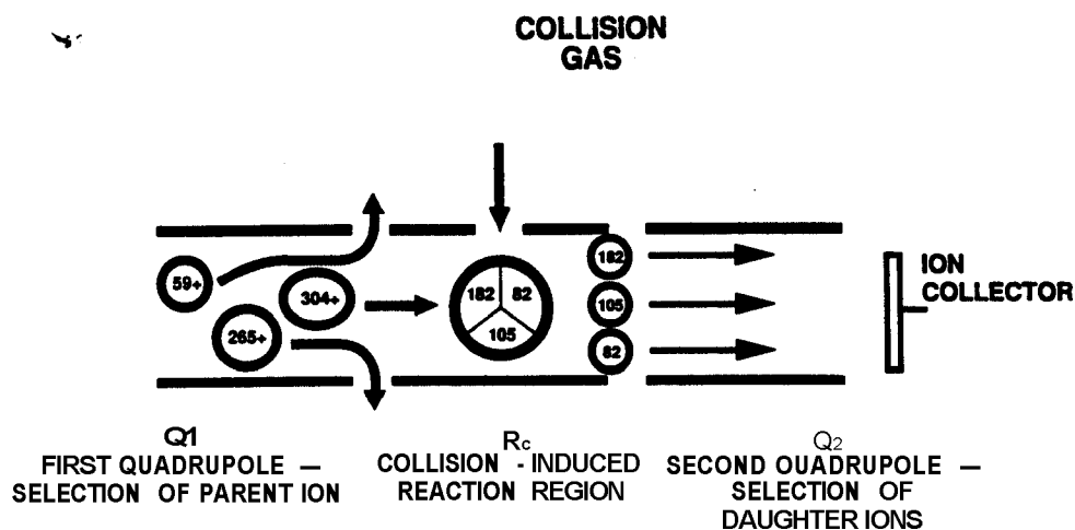
Figure 10.1. Schematic diagram of Sciex Aromic system. Reproduced with permission
