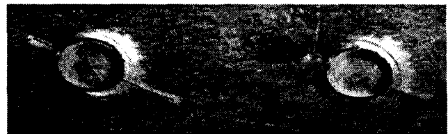
Figure 4: (a) Edge of Light image of two rivets from a Boeing 737. There are two cracks extending from each rivet. The rivet heads are about 7 mm in diameter.
