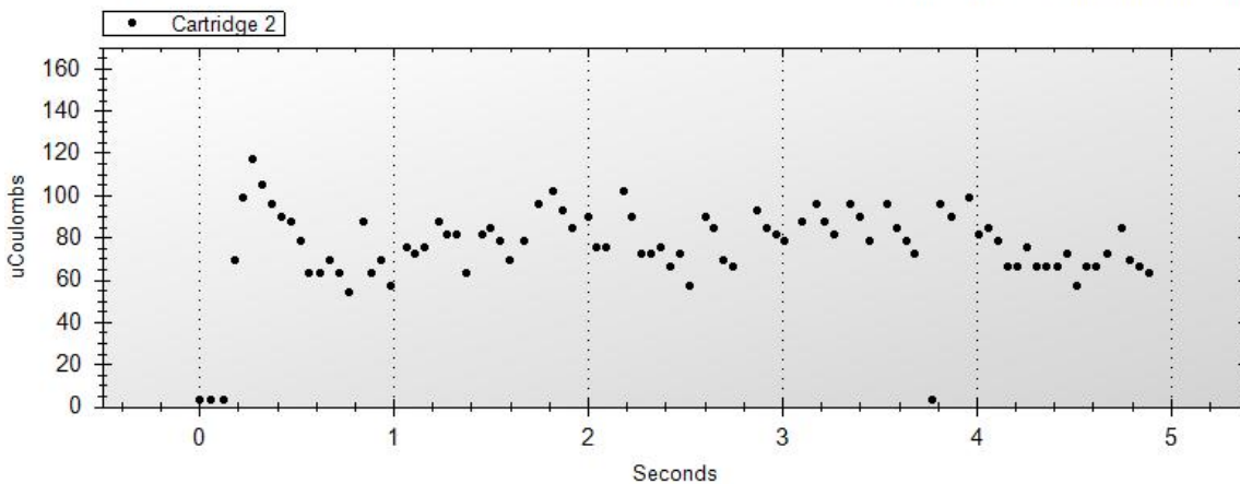
Figure 39: Charge Pulse Log for a missed shot
