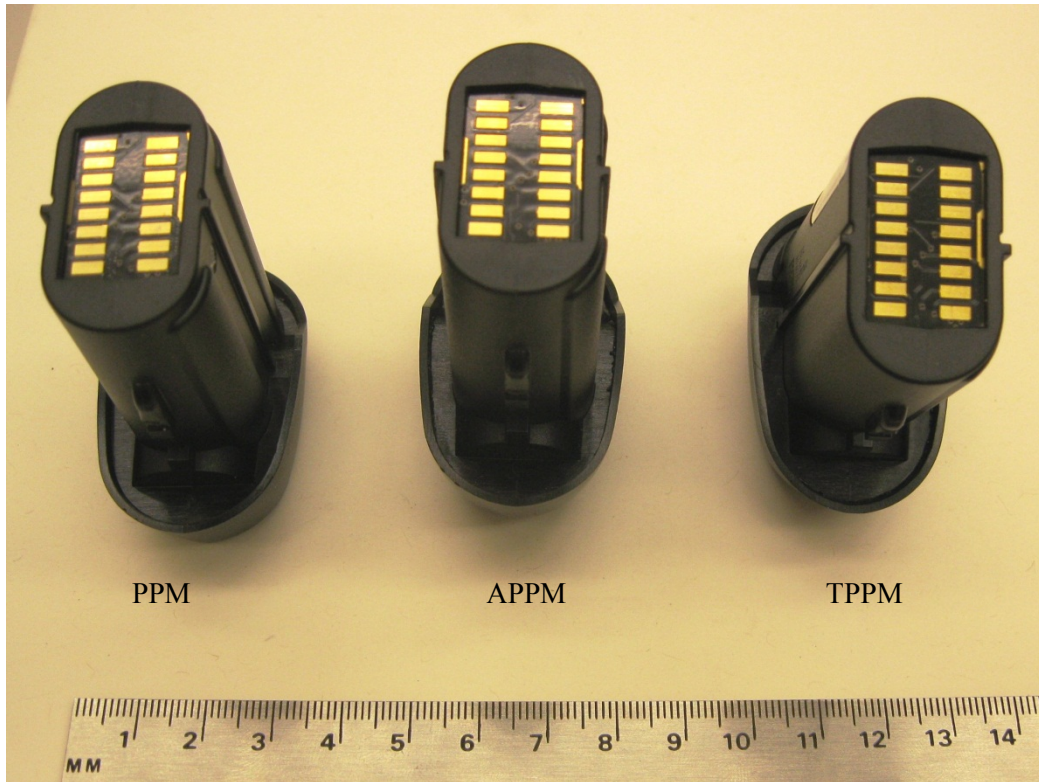
Figure 17: Contact pads on the PPMs
