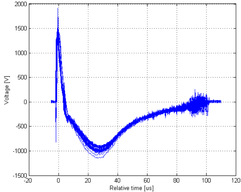
Figure 64: Overlay of all 98 pulses contained in a 5-second discharge cycle from the left-side bay
