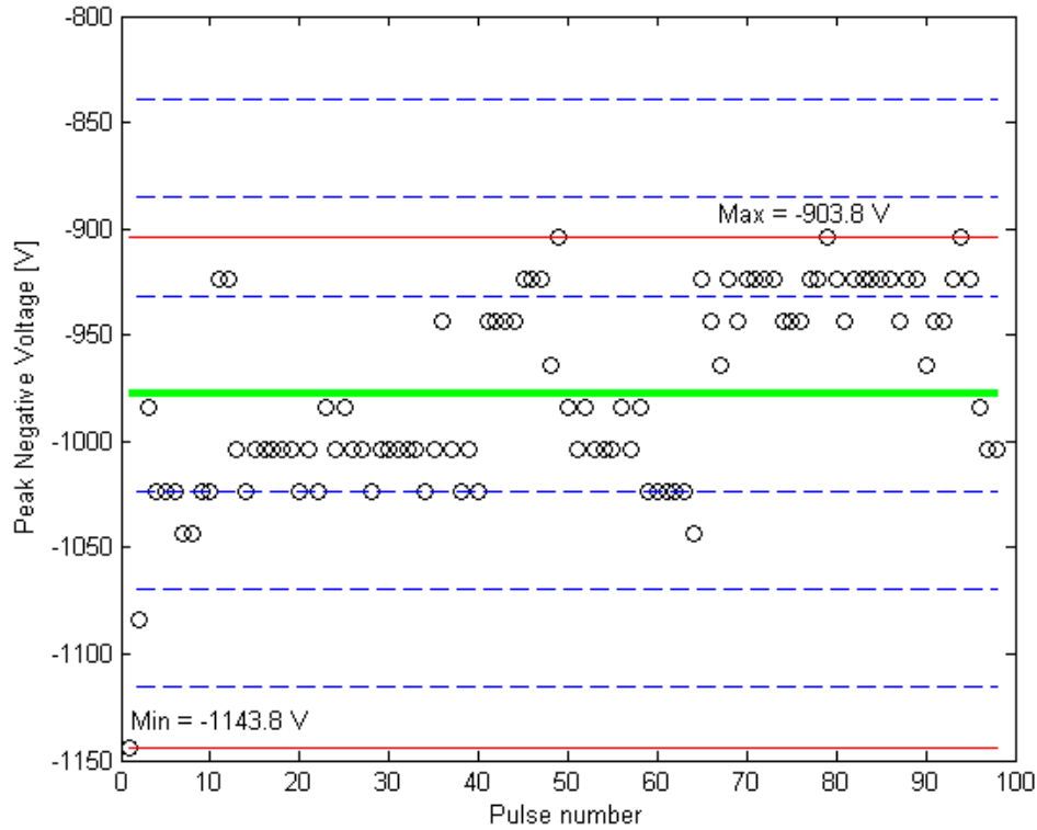
Figure 66: Main phase peak voltage of all 98 pulses contained in a 5-second discharge cycle from the left-side bay
